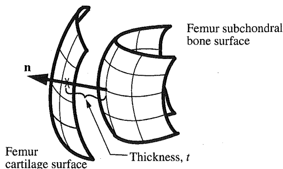
Fig. 1 The cartilage thickness is calculated by determining the intersection distance, t , along the normal, \mathbf{n} , from each resampled point on the bone surface to the cartilage surface. Alternatively, the same method may be used to find the proximity of one surface to another to estimate joint contact.
